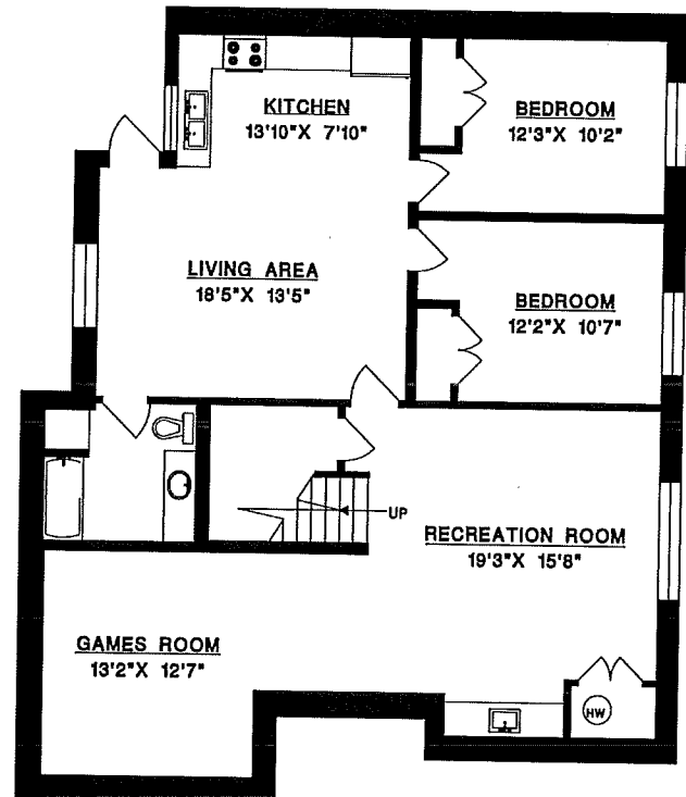
LOWER FLOOR
