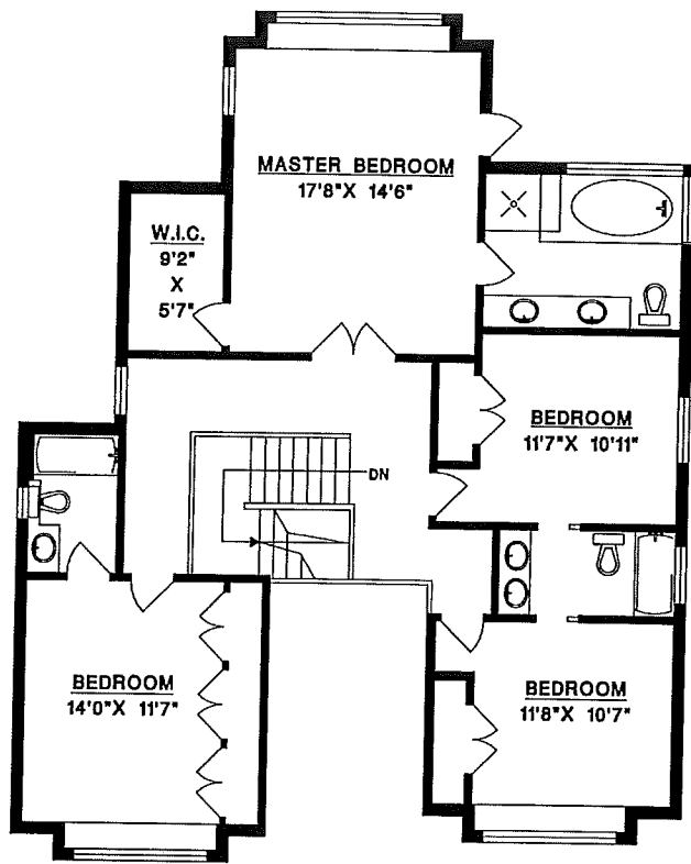
UPPER FLOOR
