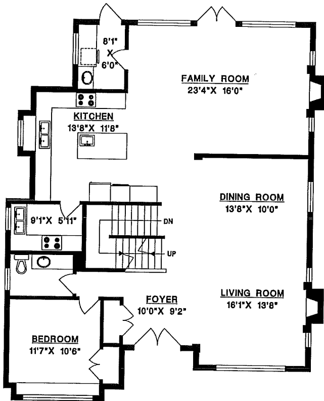
MAIN FLOOR
